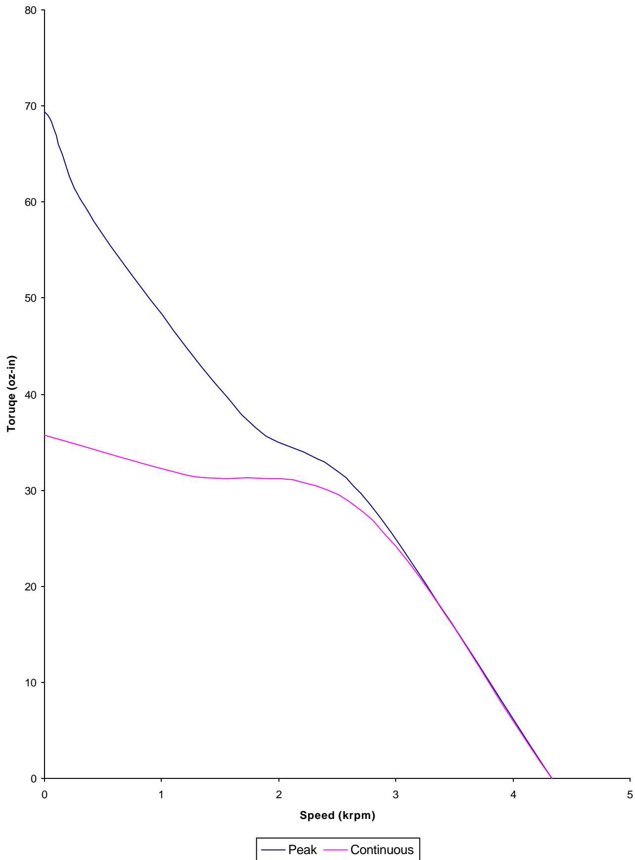
SM2337D Torque vs. Speed at 24 VDC using a PS24V8A supply
