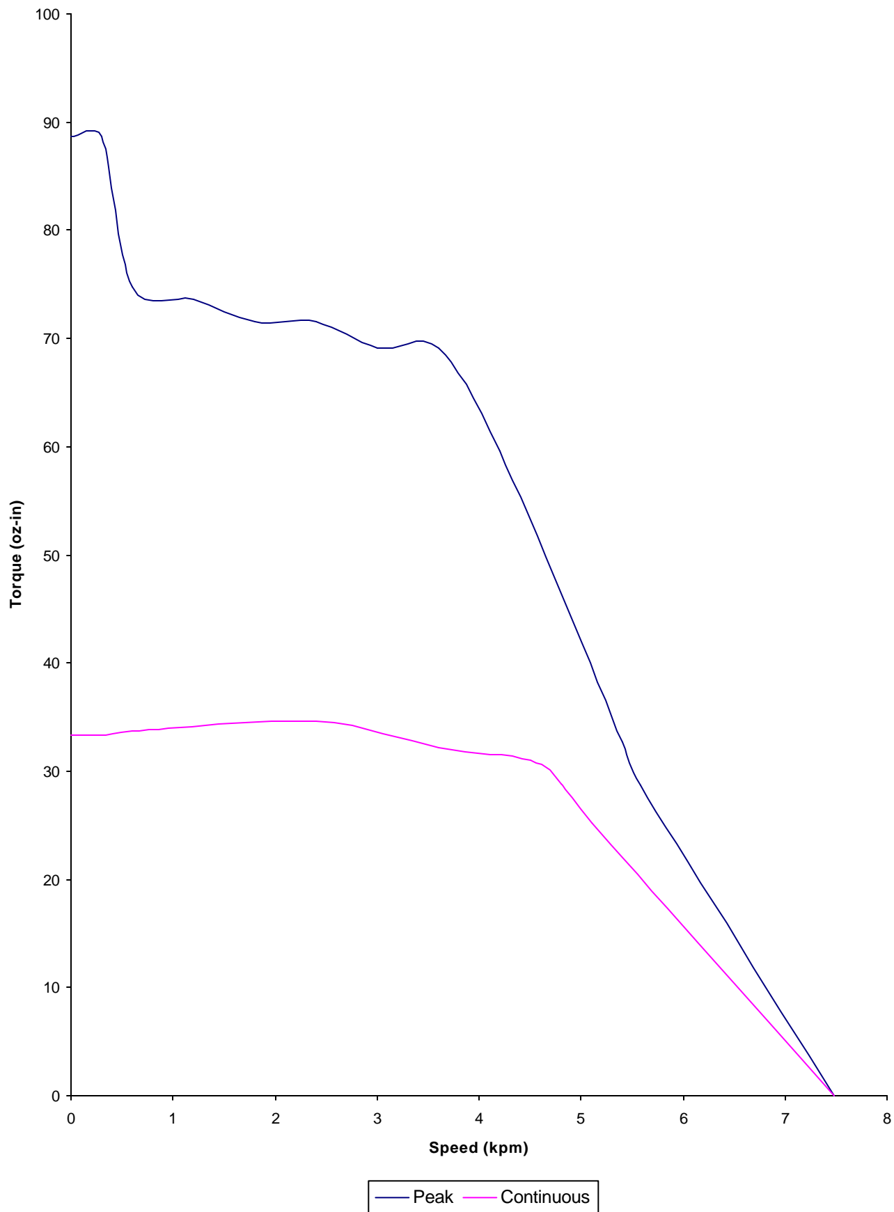
SM2337D Torque vs. Speed at 42 VDC using a PS42V20AF supply
