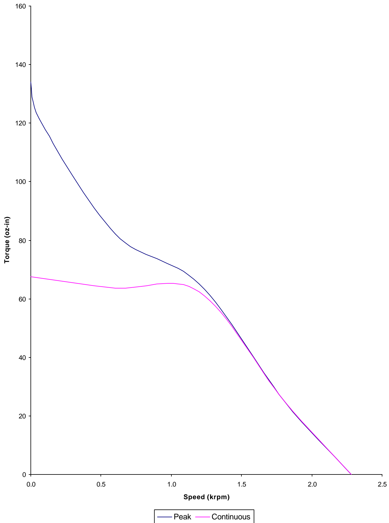
SM2337DT Torque vs. Speed at 24 VDC using a PS24V8A supply
