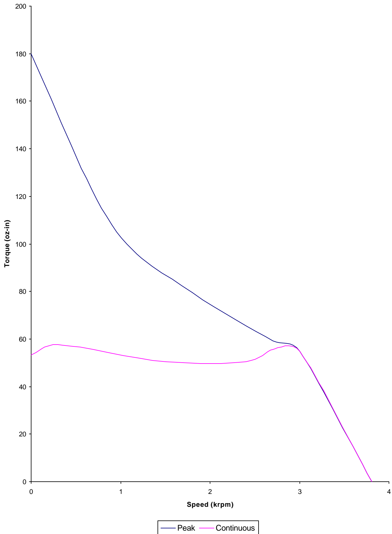
SM2337DT Torque vs. Speed at 42 VDC using a PS42V20AF supply
