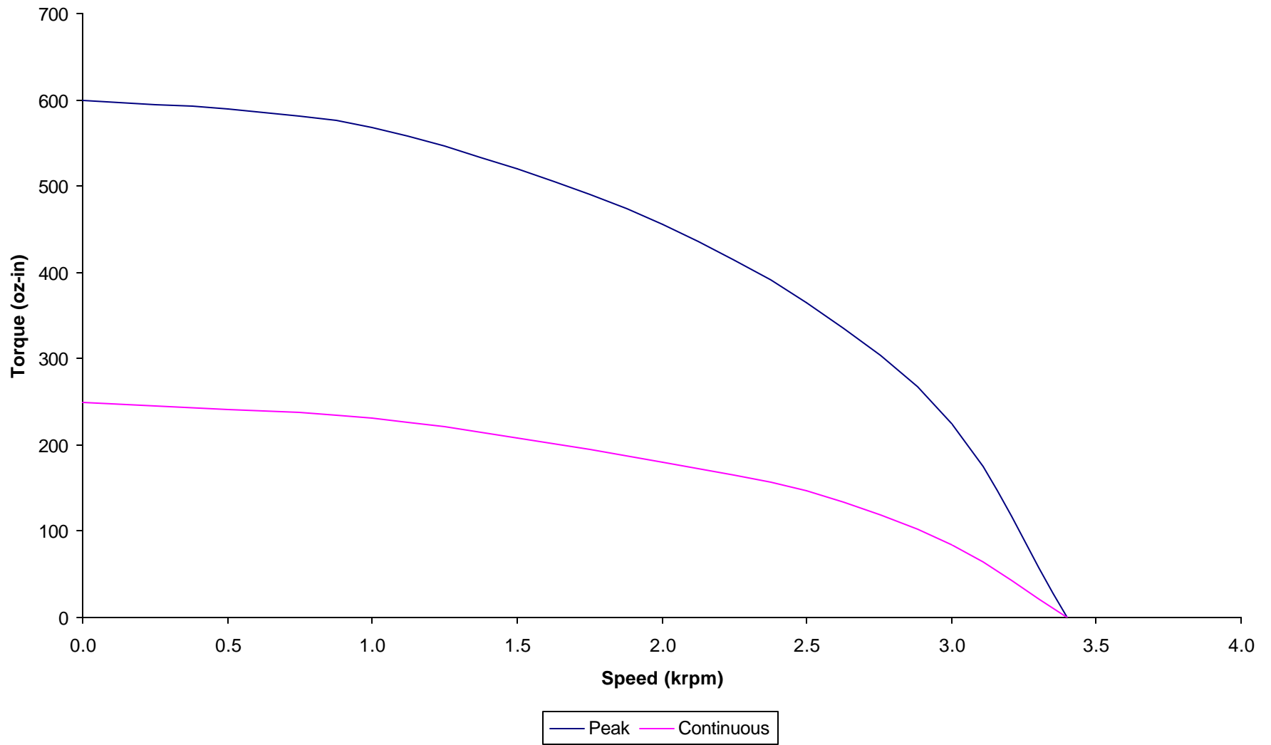
SM3450D Torque vs. Speed with 48V Battery
