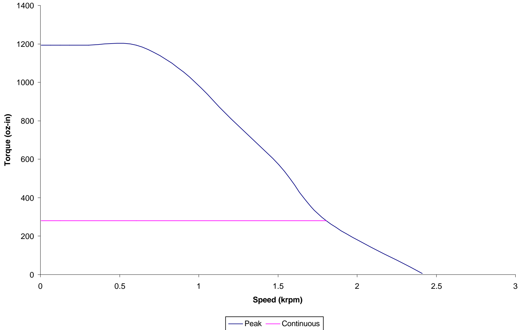
SM4210TS Torque vs. Speed with 220Vac Tri-Phase supply
