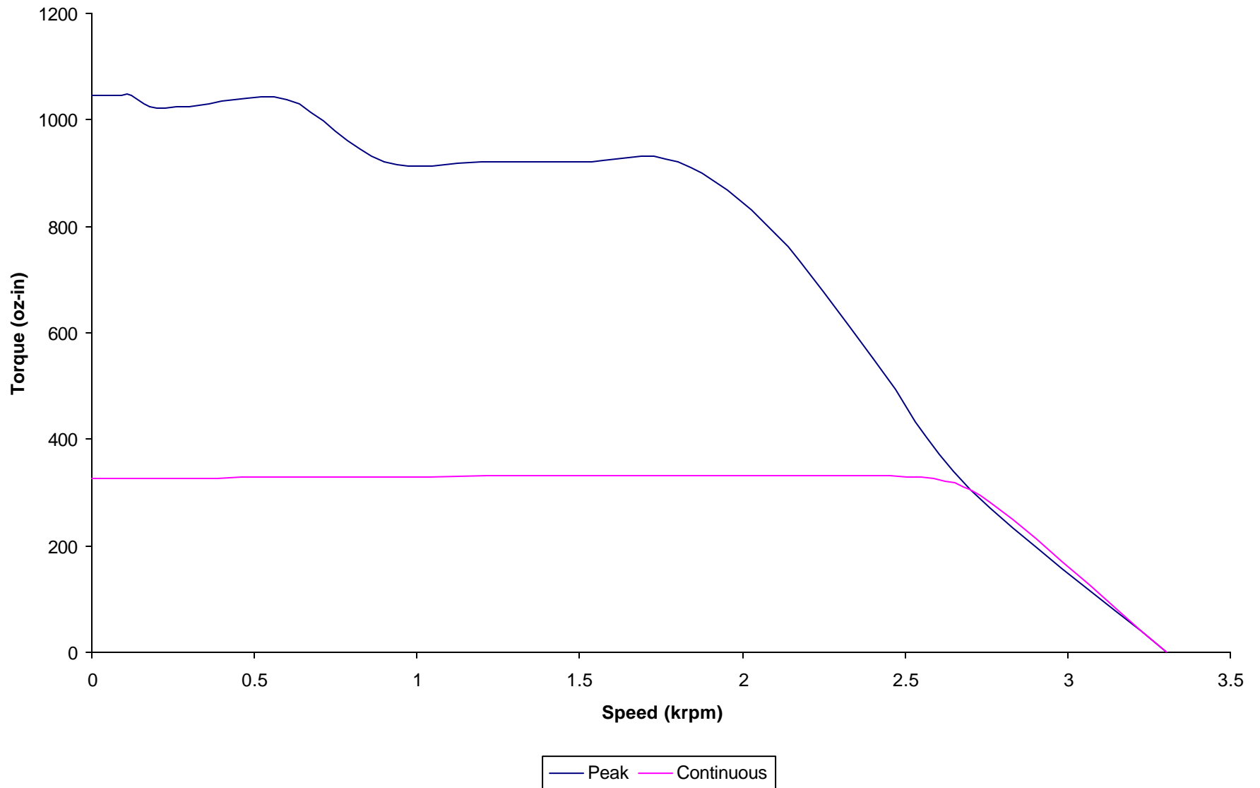
SM4220TS Torque vs. Speed with 220Vac Tri-Phase supply
