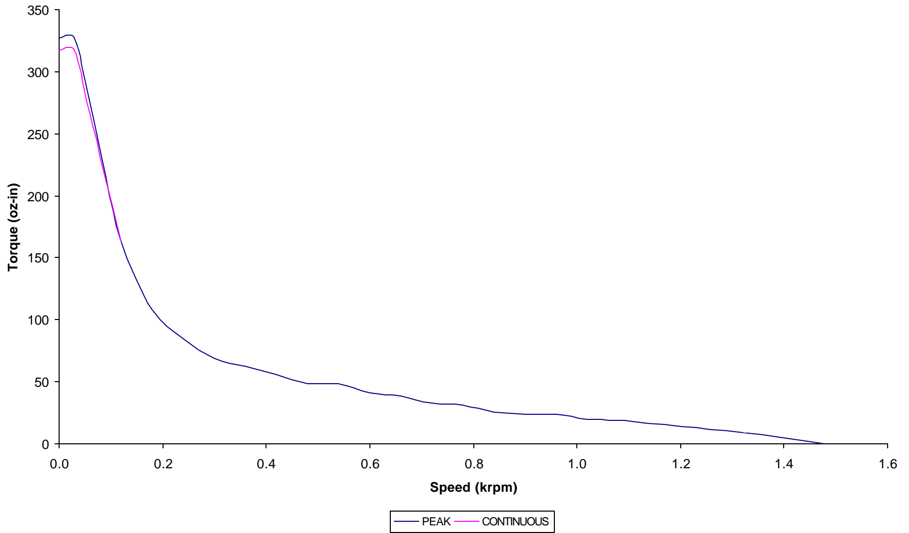
ST2340 Torque vs. Speed (24 VDC) using a PS24V8A power supply (10% Derated Torque)
