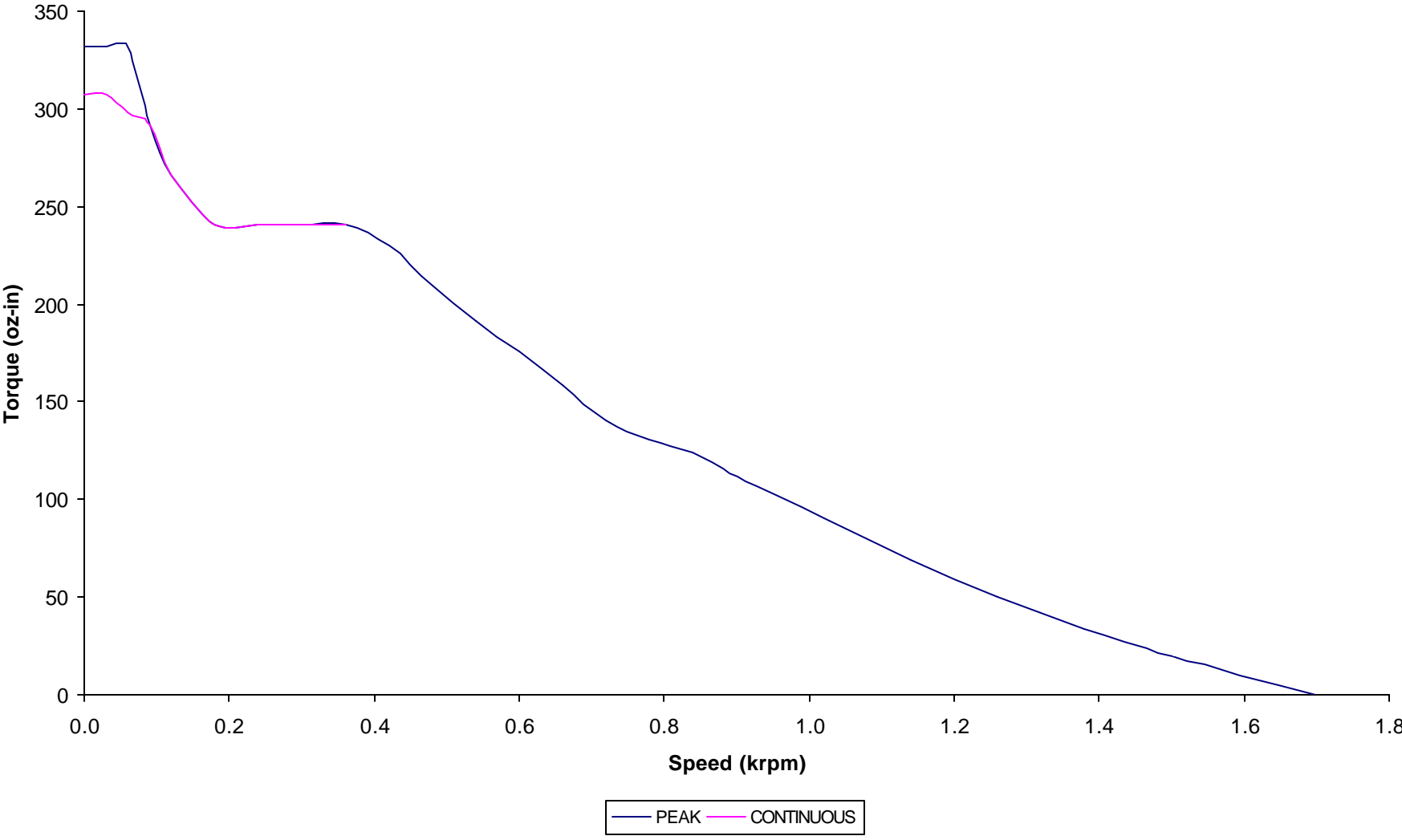
ST2340 Torque vs. Speed (75 VDC) using a PS75V6AF power supply (10% Derated Torque)
