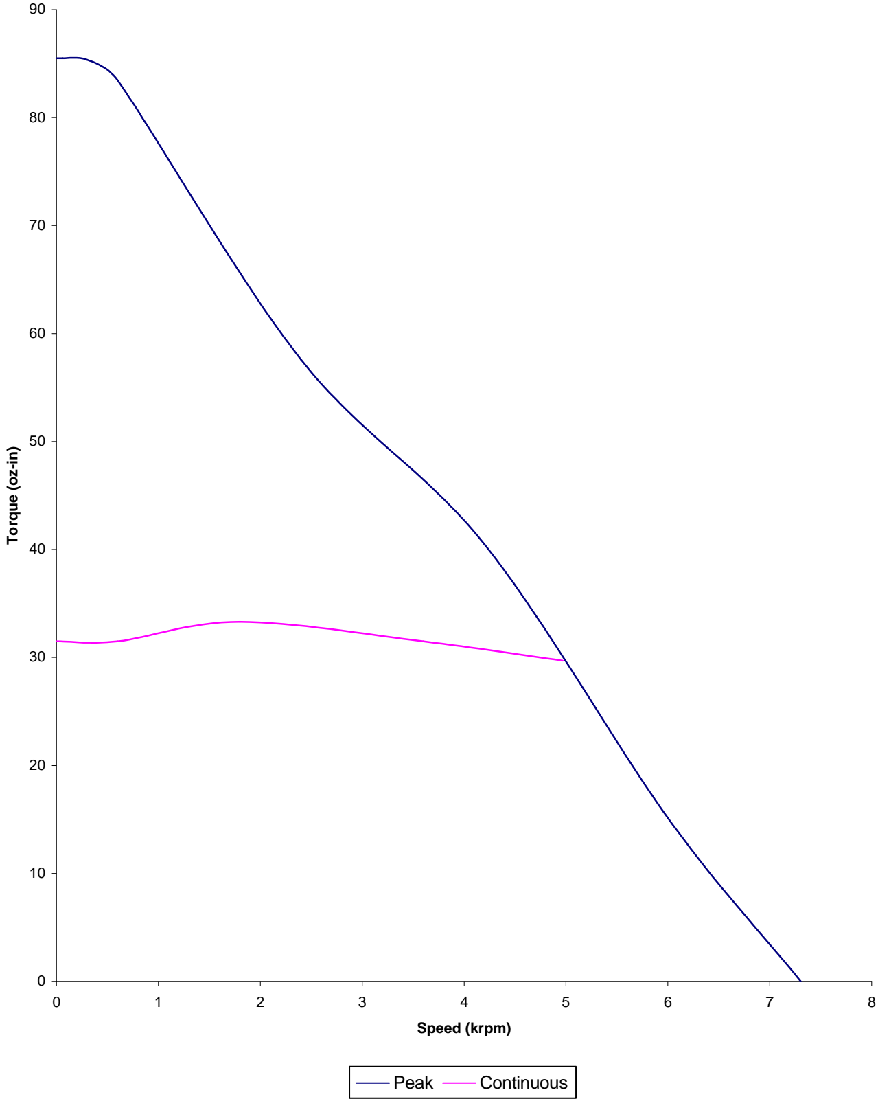
SM1720D85C Torque vs. Speed at 42 VDC using a PS42V20AF supply
