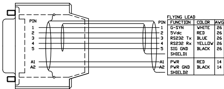
FIGURE 1: PINOUT AND COLOR CODE P1
