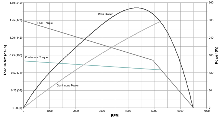
SM34166DT-BRK at 48 V at Rise from 25° to 105° C
