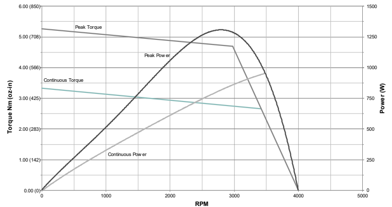
SM34266DT-BRK at 48 V at Rise from 25° to 105° C
