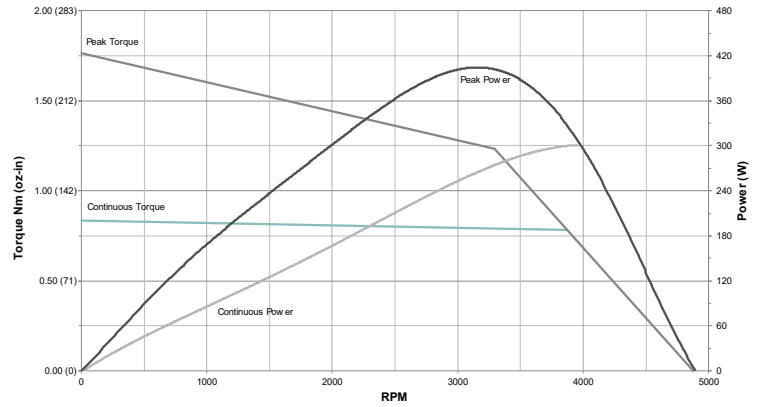
SM23266DT at 48 V at Rise from 25° to 105° C
