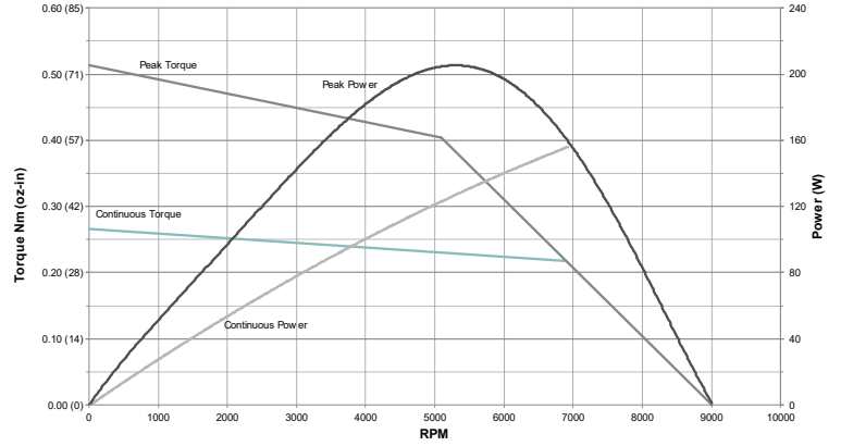
SM23166D at 48 V at Rise from 25° to 105° C
